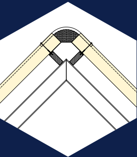
1. nokdetail
