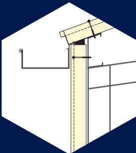
2. gootdetail
