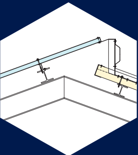
1. lichtnokdetail
